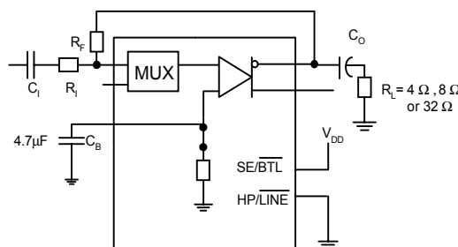
Figure 3. SE Test Circuit
