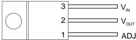
Front View for TO-220
