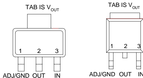
Front View for SOT-223
