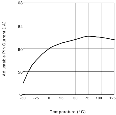
Adjustable Pin Current vs. Temperature
