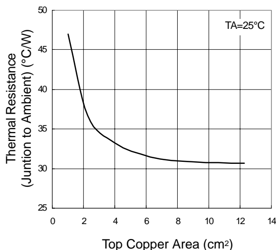
Figure 3. \theta(J-A) vs. copper area for the SOT-252 package
