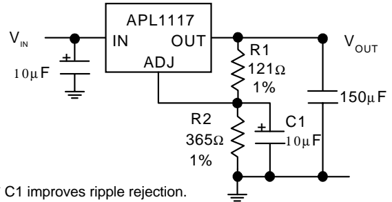
Improving Ripple Rejection
