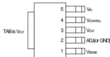
Front View of TO-252-5
