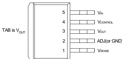
Front View of TO-263-5
