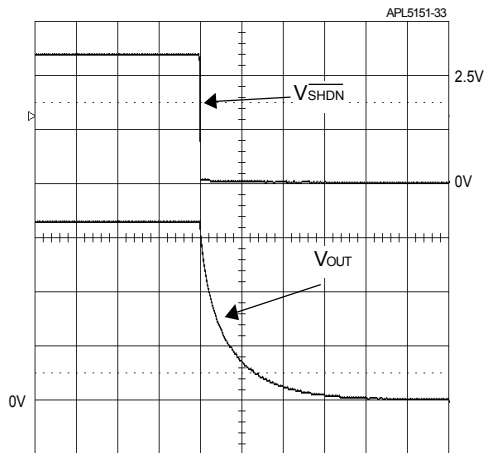
Time (0.1ms/div)
