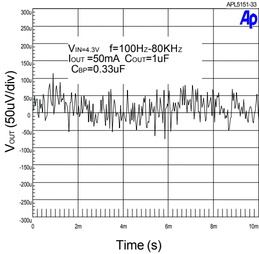
Output Noise
