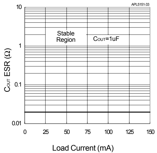
Region of Stable ESR vs. Load Current
