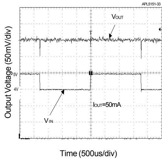
Line-Transient Response
