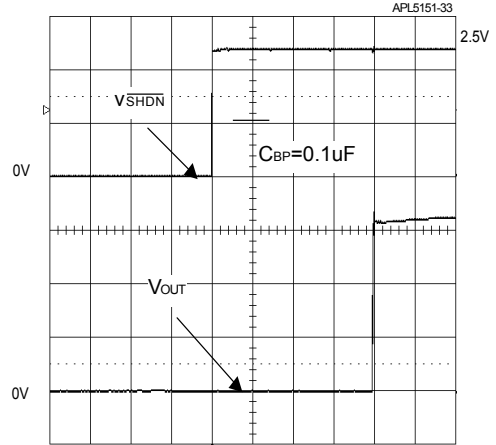
Time (1ms/div)
