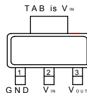
SOT-223 (Top View) APL5508
