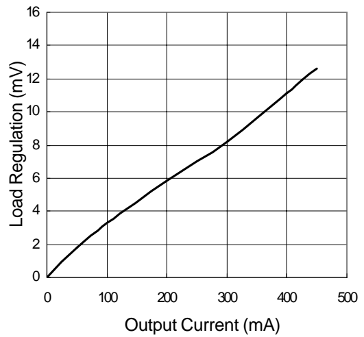
Output Current vs. Load Regulation
