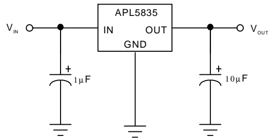
Fixed 1.8V, 2.5V, 2.6V, 2.7V, 2.8V and 3.3V Regulator
