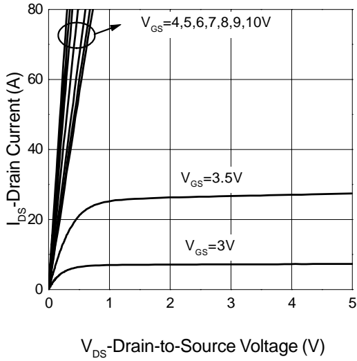
Output Characteristics
