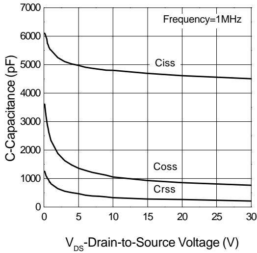
Capacitance Characteristics
