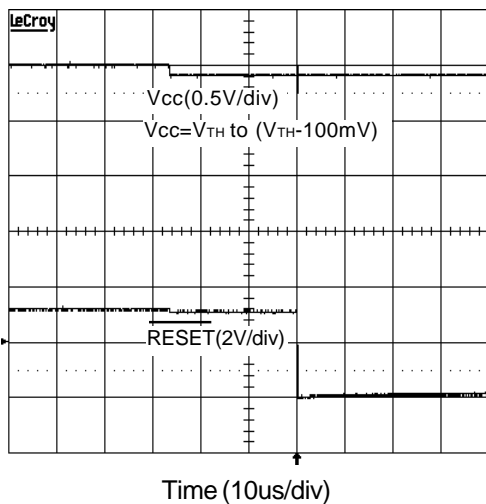
Vcc to RESET Delay
