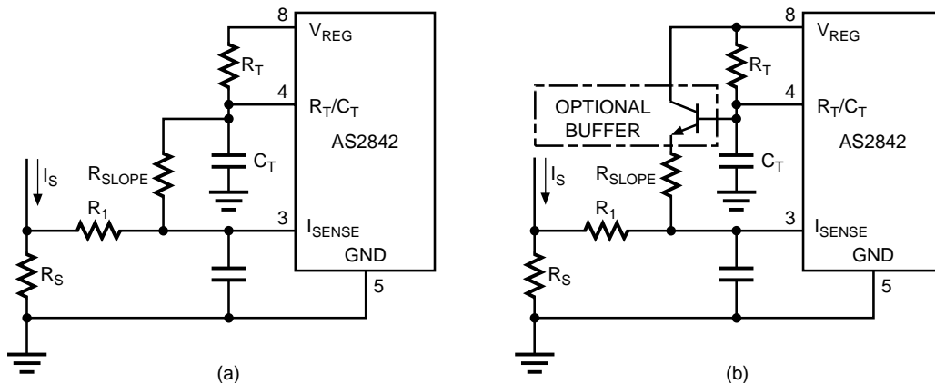
Figure 23. Slope Compensation
