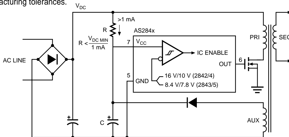
Figure 14. Bootstrap Circuit
