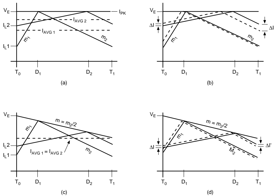
Figure 22. Slope Compensation
