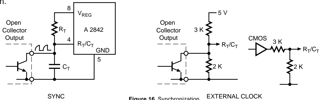
Figure 16. Synchronization
