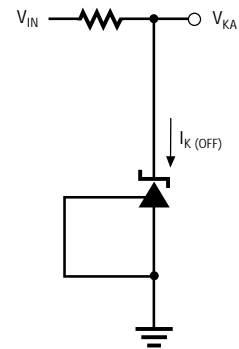
Figure 1c. Test Circuit 3
