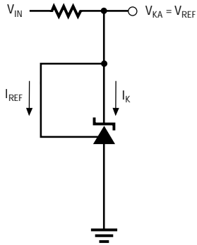
Figure 1a. Test Circuit 1
