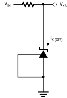
Figure 1c. Test Circuit 3
