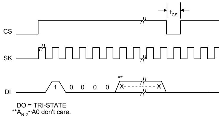
FIGURE 5. WRITE DISABLE(WDS) CYCLE TIMING
