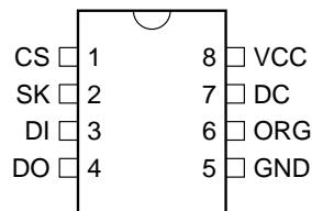
8-Pin PDIP
