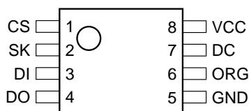
8-Pin TSSOP
