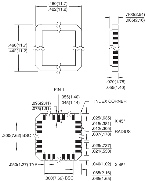
28L, 28-Pad, Non-Windowed, Ceramic Leadless Chip Carrier (LCC) Dimensions in Inches and (Millimeters) MIL-STD-1835 C-4
