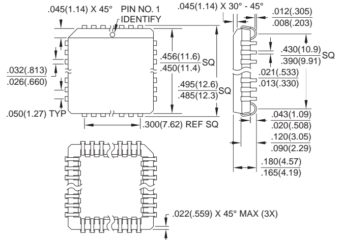
28J, 28-Lead, Plastic J-Leaded Chip Carrier (PLCC) Dimensions in Inches and (Millimeters) JEDEC STANDARD MS-018 AB
