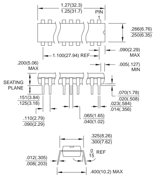
24P3, 24-Lead, 0.300" Wide, Plastic Dual Inline Package (PDIP) Dimensions in Inches and (Millimeters) JEDEC STANDARD MS-001 AF
