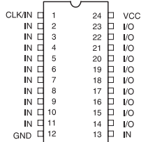
DIP/SOIC
