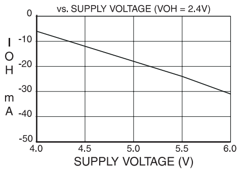
OUTPUT SOURCE CURRENT
