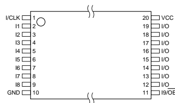
DIP/SOIC
