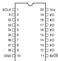
DIP/SOIC
