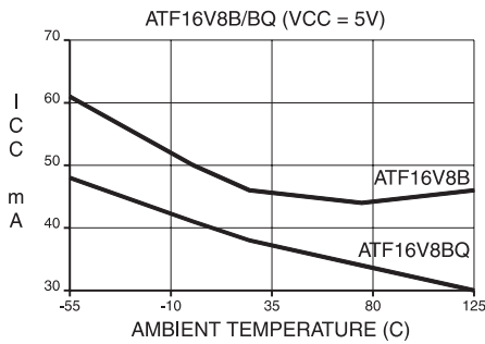
SUPPLY CURRENT vs. AMBIENT TEMPERATURE
