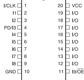
DIP/SOIC
