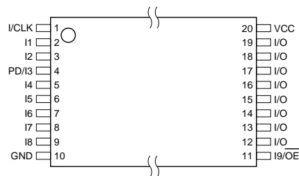
DIP/SOIC
