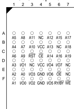
CBGA Top View
