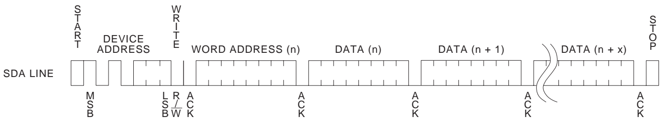
Figure 3. Page write
