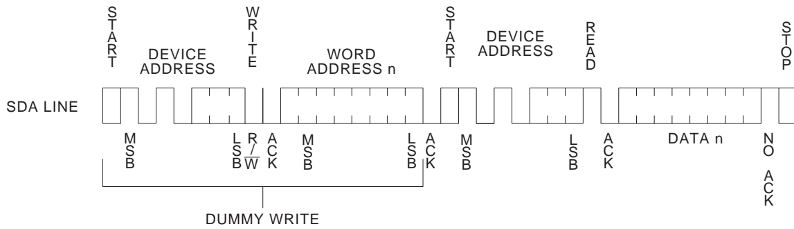
Figure 5. Random Read
