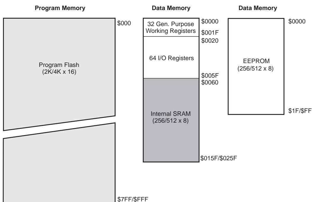
Figure 4. Memory Maps
