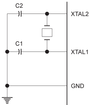
Figure 1. Oscillator Connections
