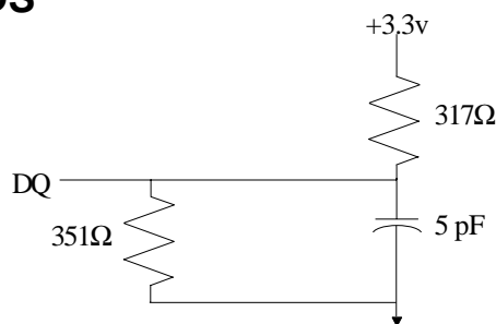
Fig. 2 3.3V I/O OUTPUT LOAD EQUIVALENT
