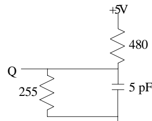
Fig. 2 Output Load Equivalent
