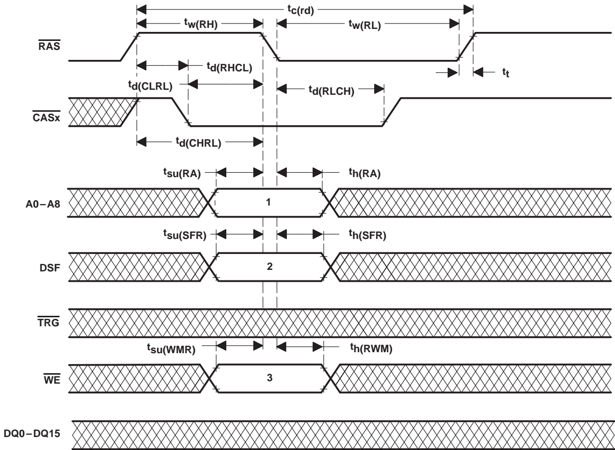
Figure 44. CBR-Refresh-Cycle Timing
