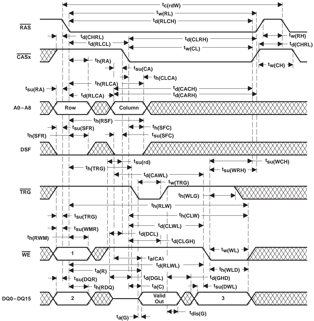
Figure 33. Read-Write-/Read-Modify-Write-Cycle Timing
