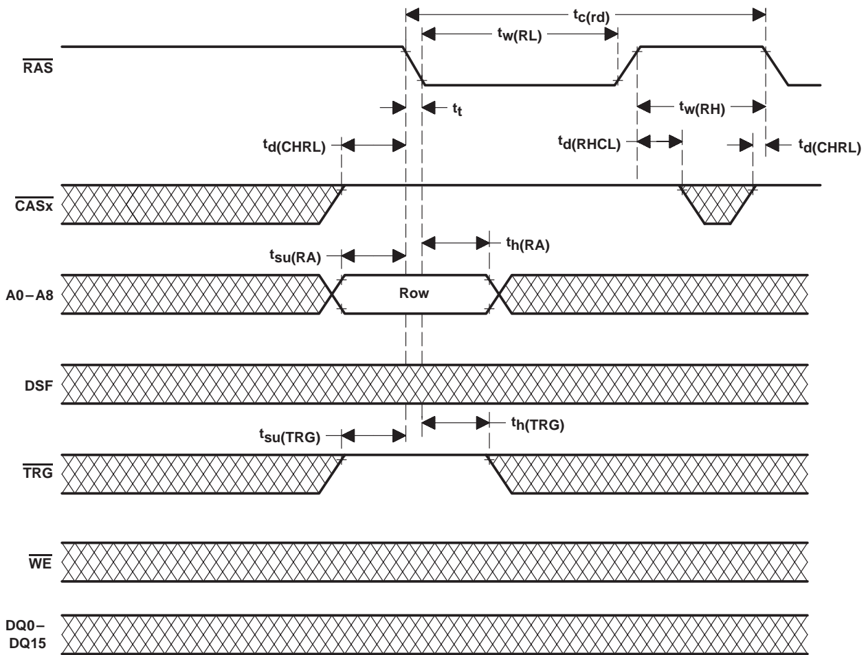
Figure 43. RAS-Only Refresh-Cycle Timing
