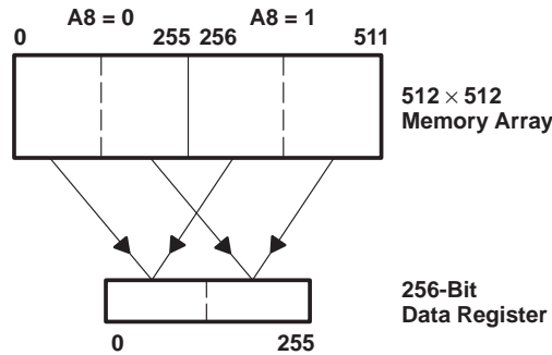
Figure 17. Split-Register-Transfer Read
