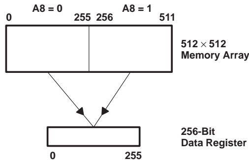
Figure 15. Full-Register-Transfer Read
