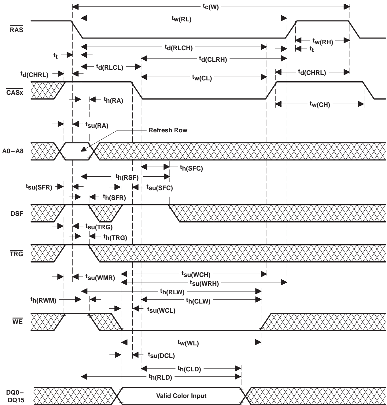
Figure 38. Load-Color-Register-Cycle Timing (Early-Write Load)
