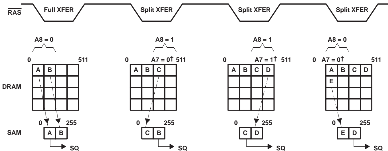
Figure 18. Example of a Split-Register-Transfer Read Operation
