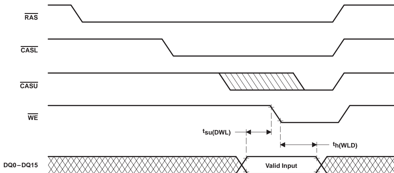
Figure 6. Example of a Late-Write Cycle
