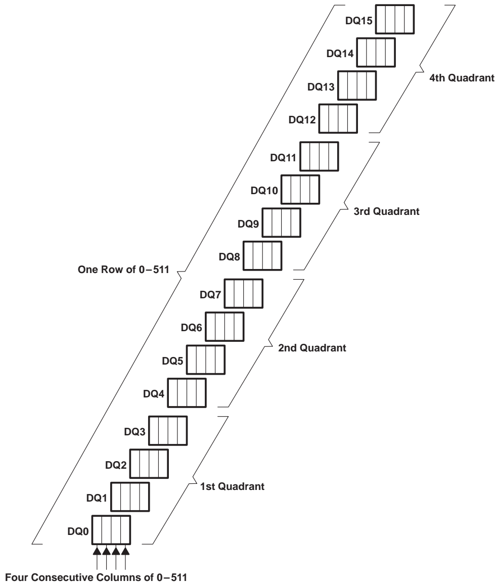
Figure 9. Block-Write Operation
