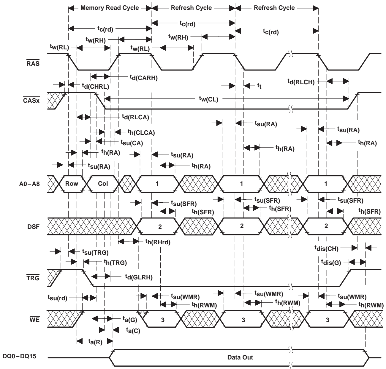
Figure 45. Hidden-Refresh-Cycle Timing
