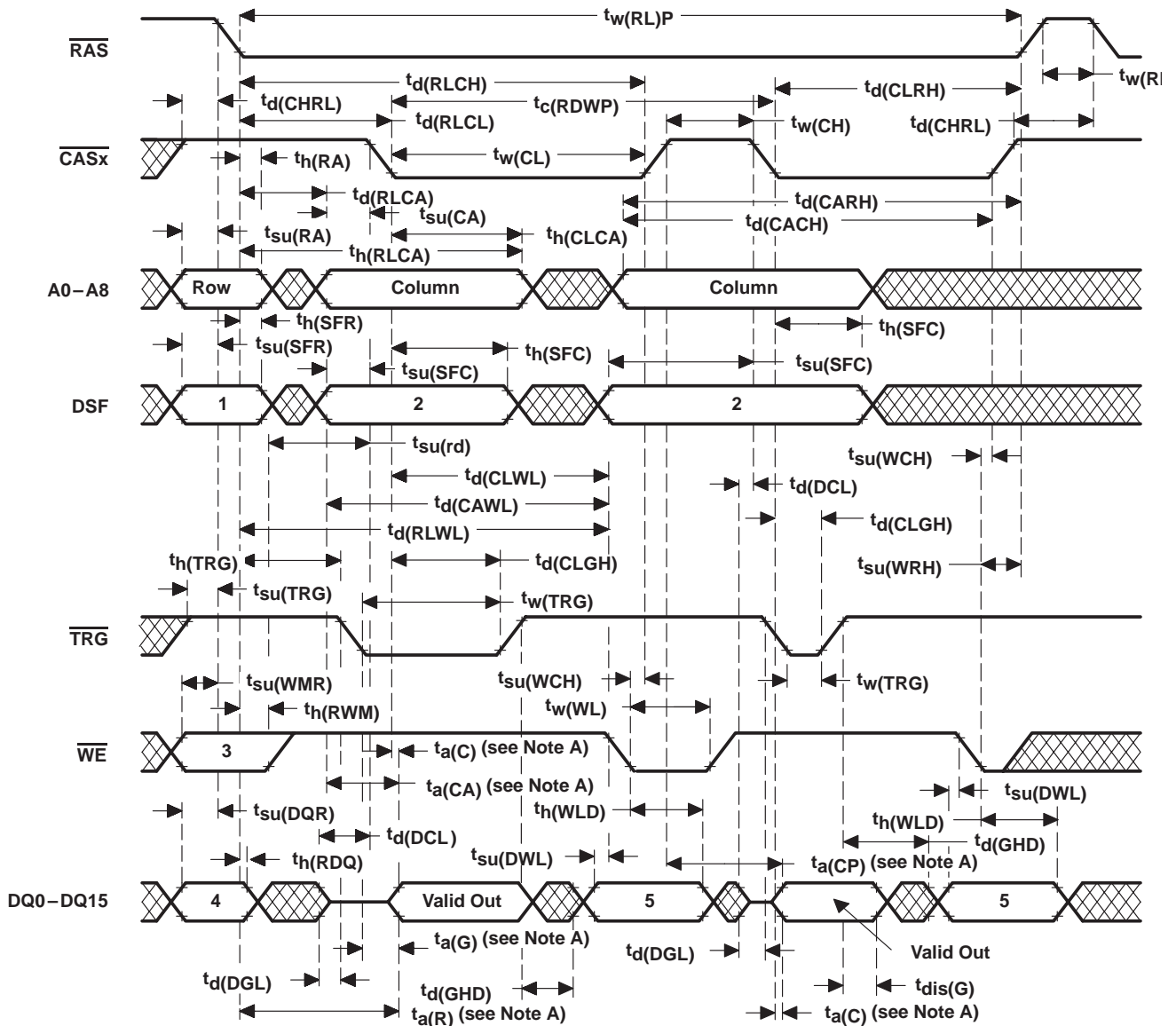
Figure 36. Enhanced-Page-Mode Read-Modify-Write-Cycle Timing Table 11. Enhanced-Page-Mode Read-Modify-Write-Cycle State Table
