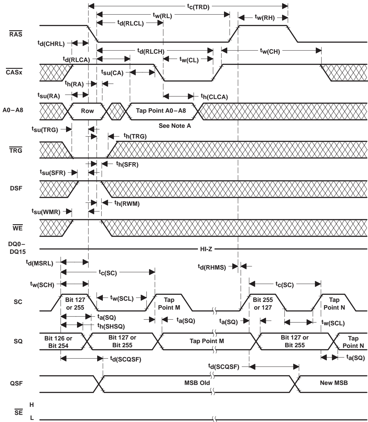
Figure 48. Split-Register-Transfer-Read Timing
