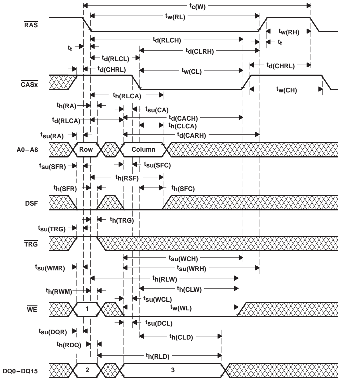
Figure 29. Early-Write-Cycle Timing
