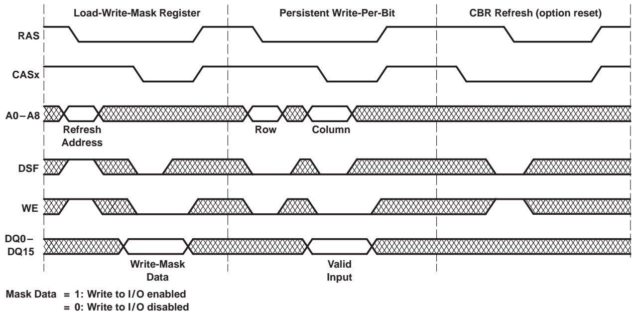
Figure 8. Example of a Persistent Write-Per-Bit Operation
