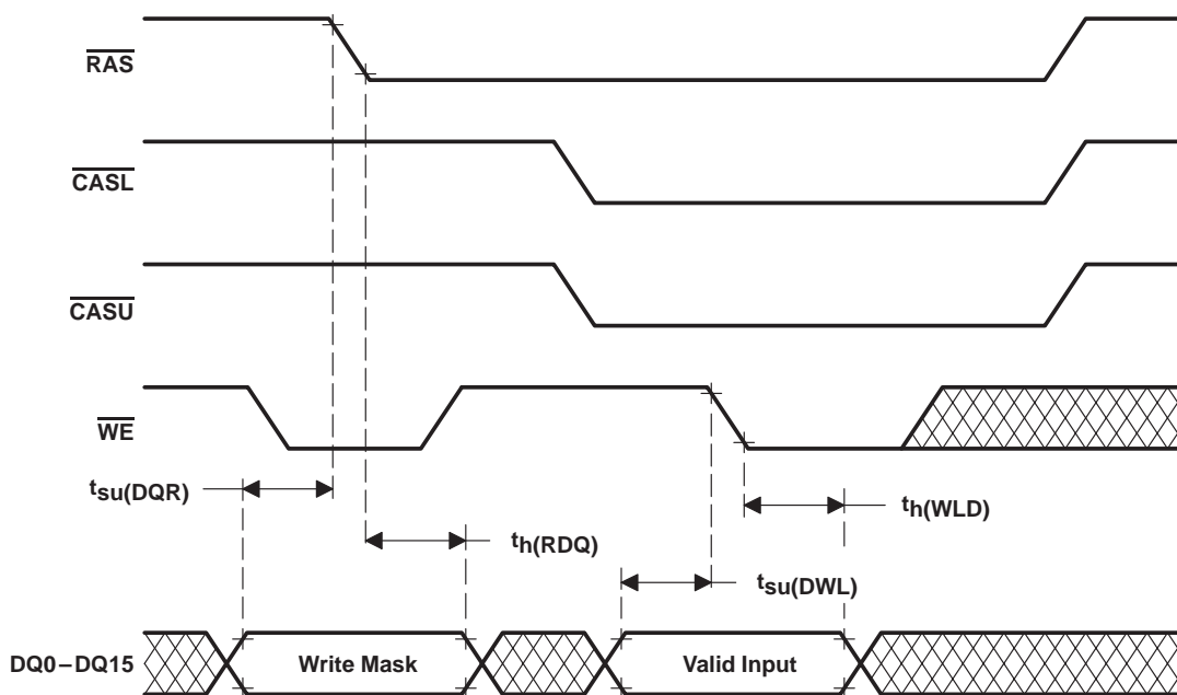
Figure 7. Example of a Nonpersistent Write-Per-Bit (Late-Write) Operation
