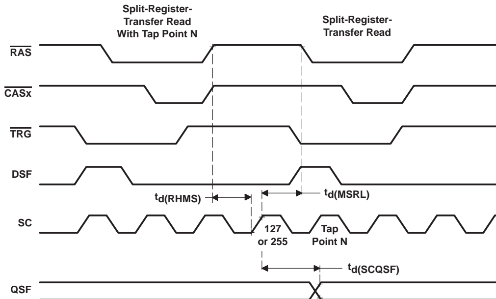
Figure 20. Example of Successive Split-Register-Transfer-Read Operations
