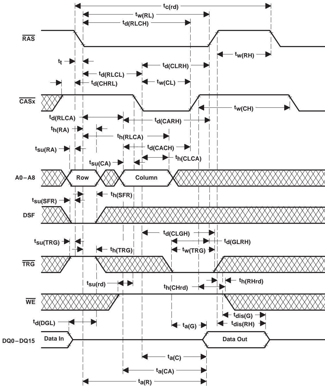
Figure 28. Read-Cycle Timing With \overline{RAS} -Controlled Output
