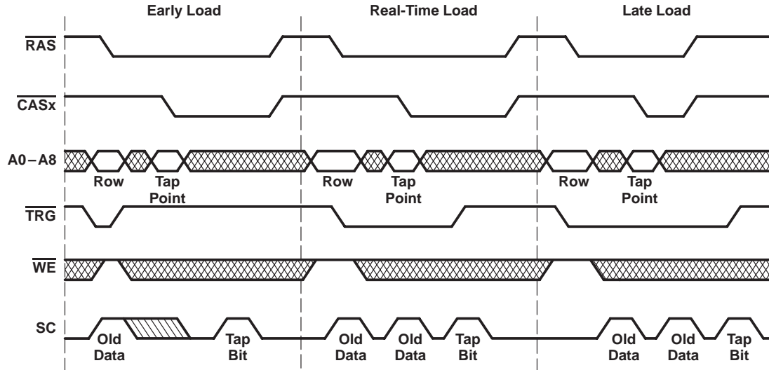
Figure 16. Example of Full-Register-Transfer Read Operations
