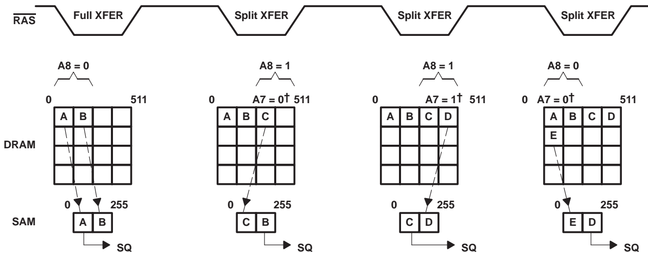
Figure 17. Example of a Split-Register-Transfer Read Operation
