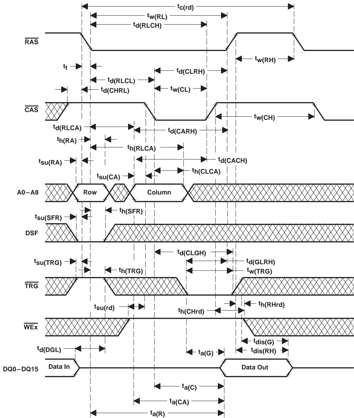
Figure 27. Read-Cycle Timing With \overline{RAS} -Controlled Output
