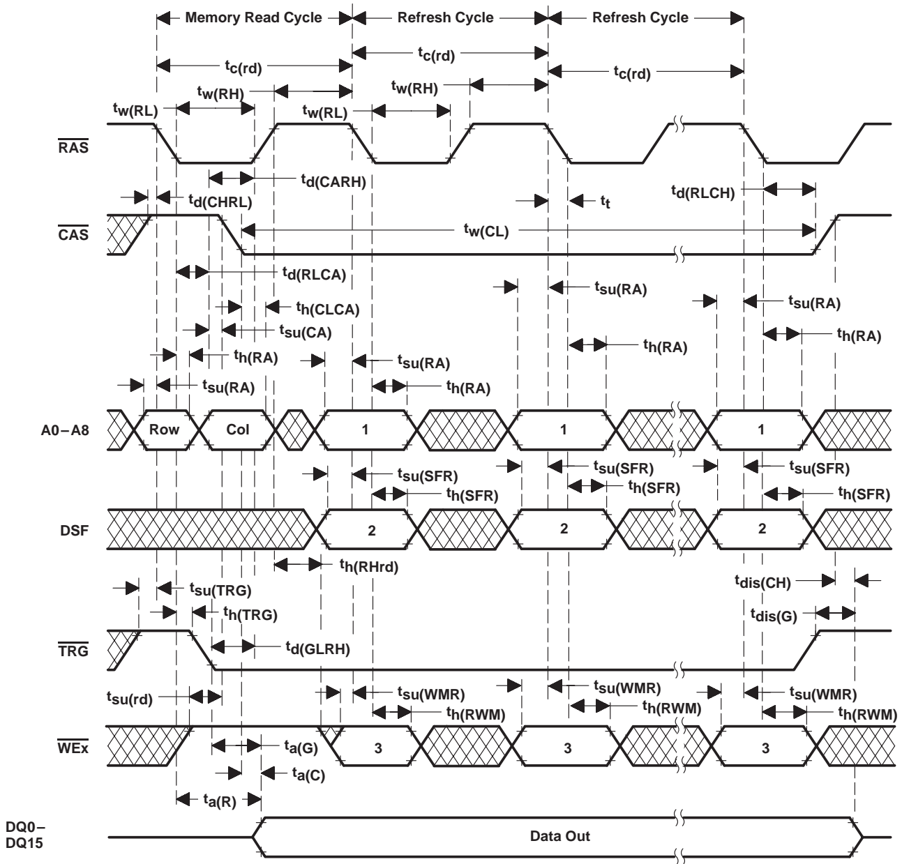
Figure 44. Hidden-Refresh-Cycle Timing
