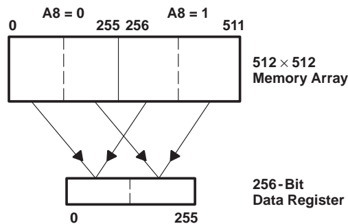
Figure 16. Split-Register-Transfer Read
