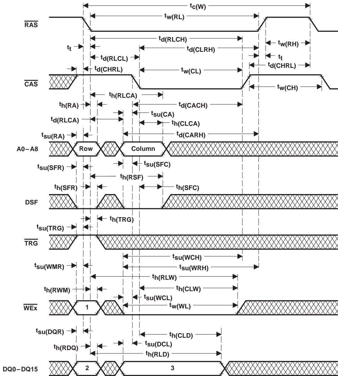
Figure 28. Early-Write-Cycle Timing
