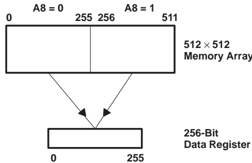
Figure 14. Full-Register-Transfer Read
