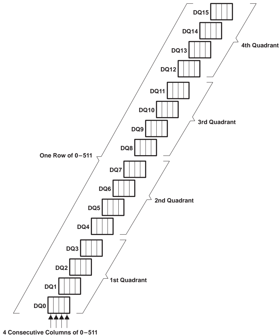
Figure 8. Block-Write Operation
