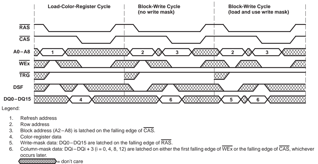
Figure 12. Example of Block Writes
