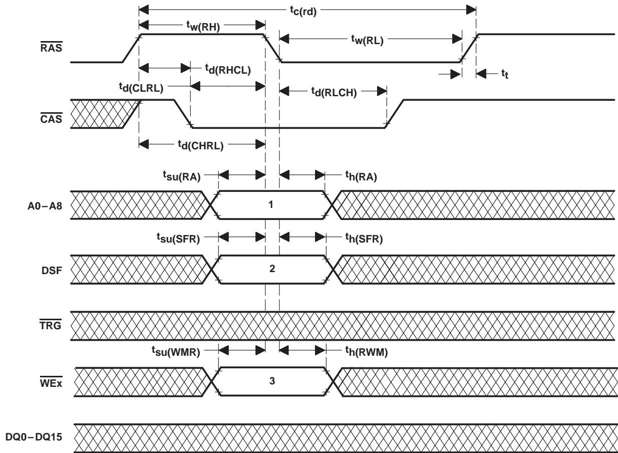
Figure 43. CBR-Refresh-Cycle Timing
