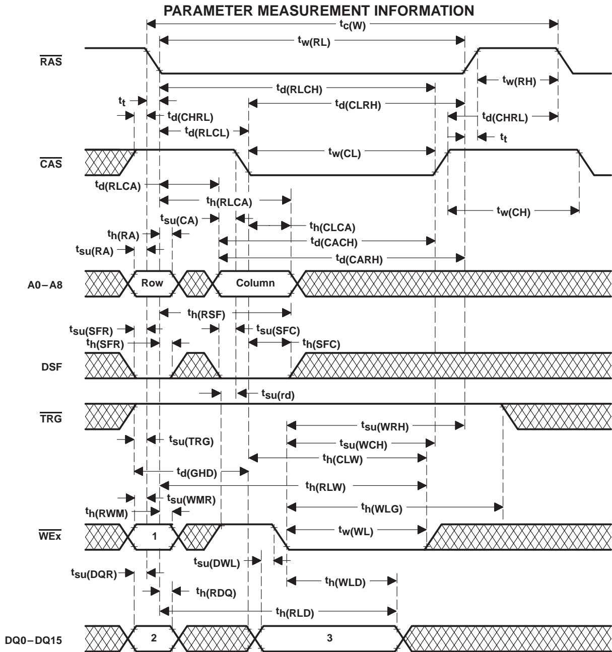
Figure 29. Late-Write-Cycle Timing (Output-Enable-Controlled Write)
