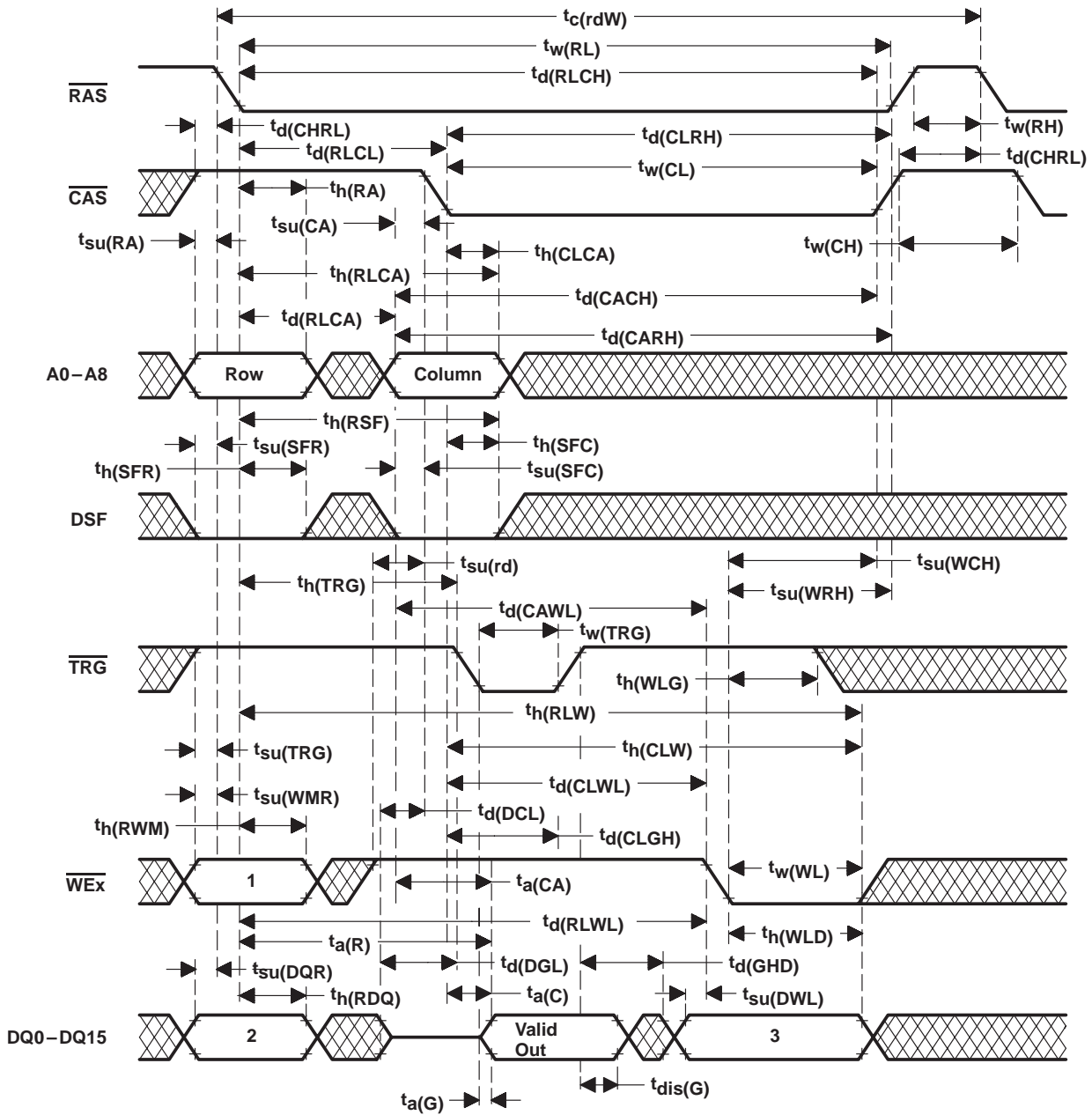
Figure 32. Read-Write-/Read-Modify-Write-Cycle Timing
