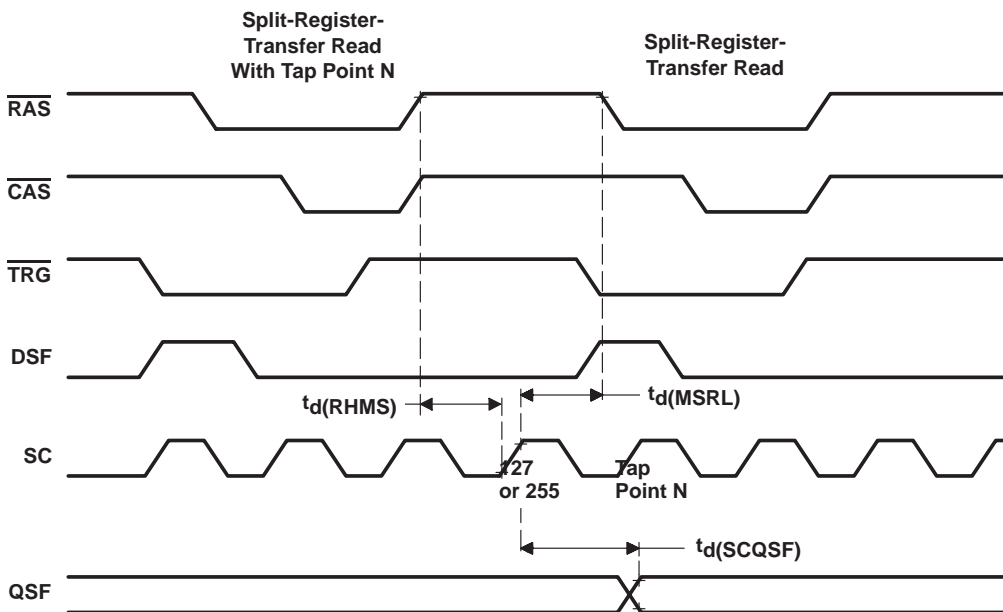
Figure 19. Example of Successive Split-Register-Transfer Read Operations
