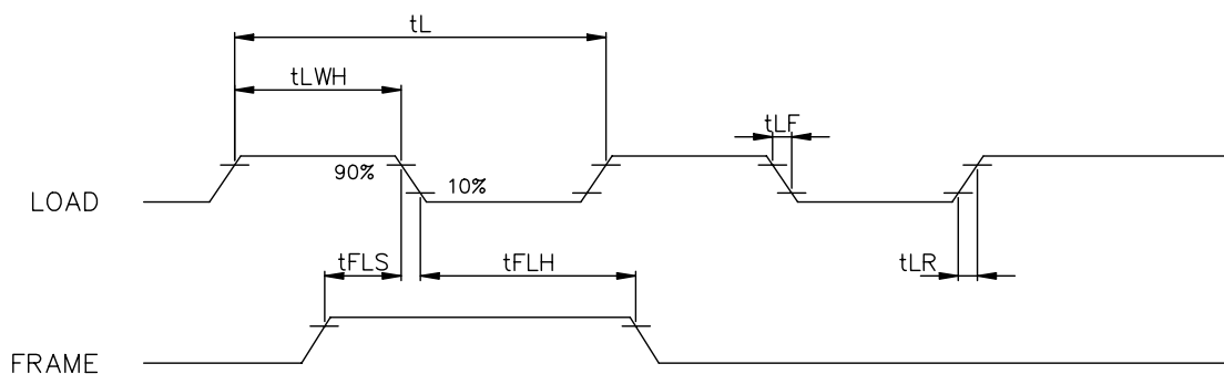
Fig . b Interface timing (COMMON)
