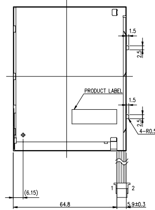
CN3 FOR TOUCH PANEL
