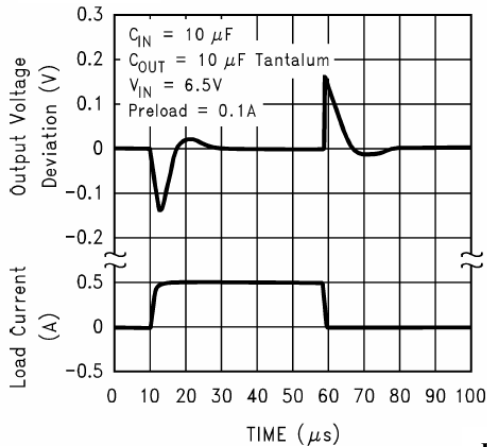
B033-5.0 Load Transient Response
