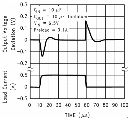
B1117-5.0 Load Transient Response
