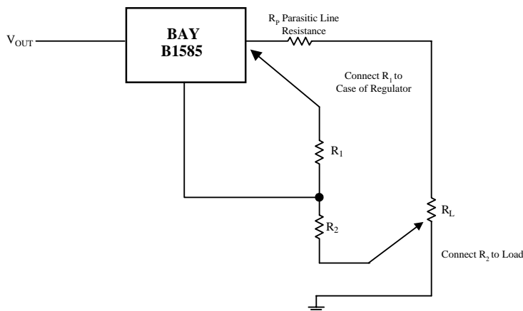
Fig.3 Basic Adjustable Regulator
