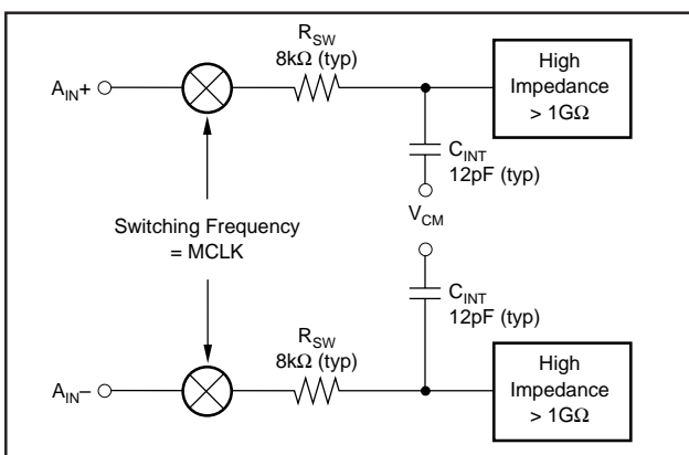
FIGURE 3. Input Impedance of the ADS1201.
