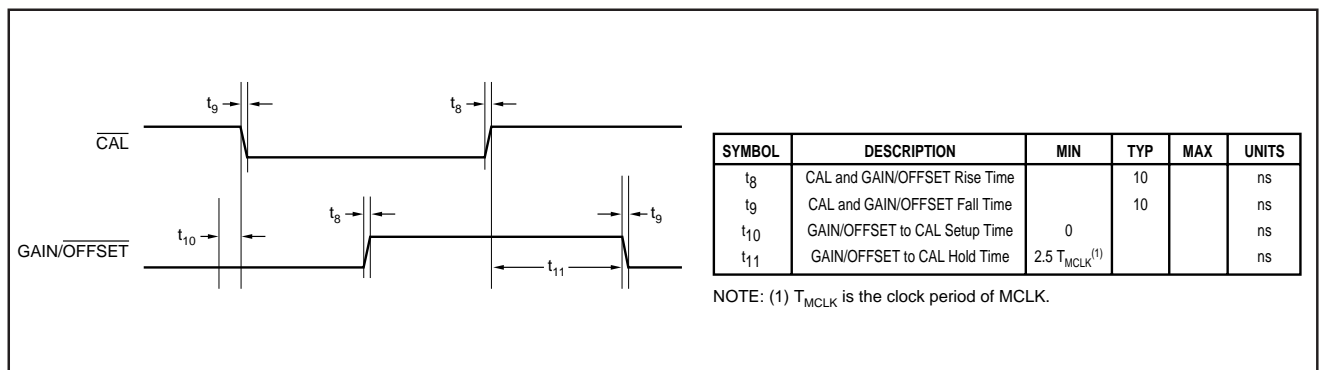
FIGURE 9. Timing Diagram for the Calibration Feature of the ADS1201.
