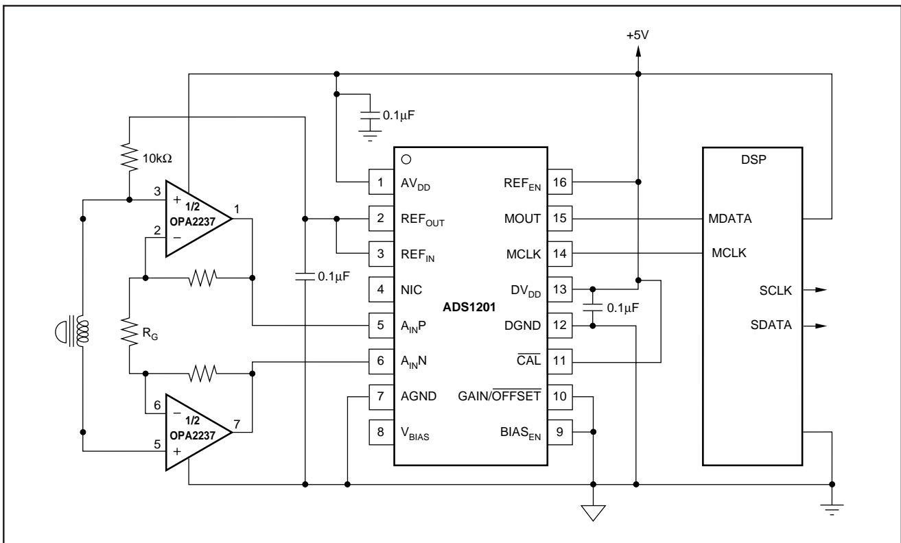
FIGURE 13. Geophone Interface.
