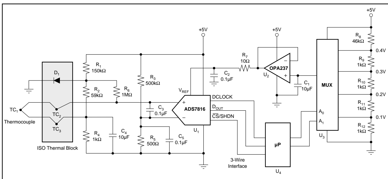
FIGURE 6. Thermocouple Application Using a MUX to Scale the Input Range of the ADS7816.
