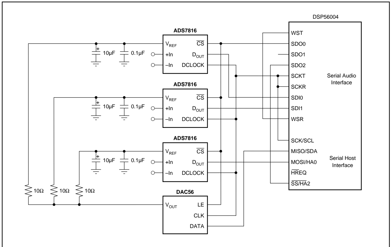
FIGURE 7. Flexible Data Acquisition System.
