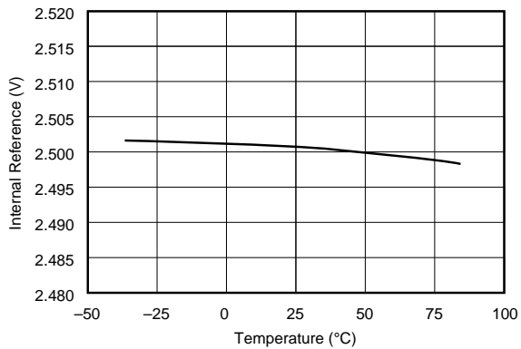
INTERNAL REFERENCE VOLTAGE vs TEMPERATURE
