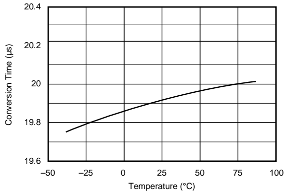
CONVERSION TIME vs TEMPERATURE
