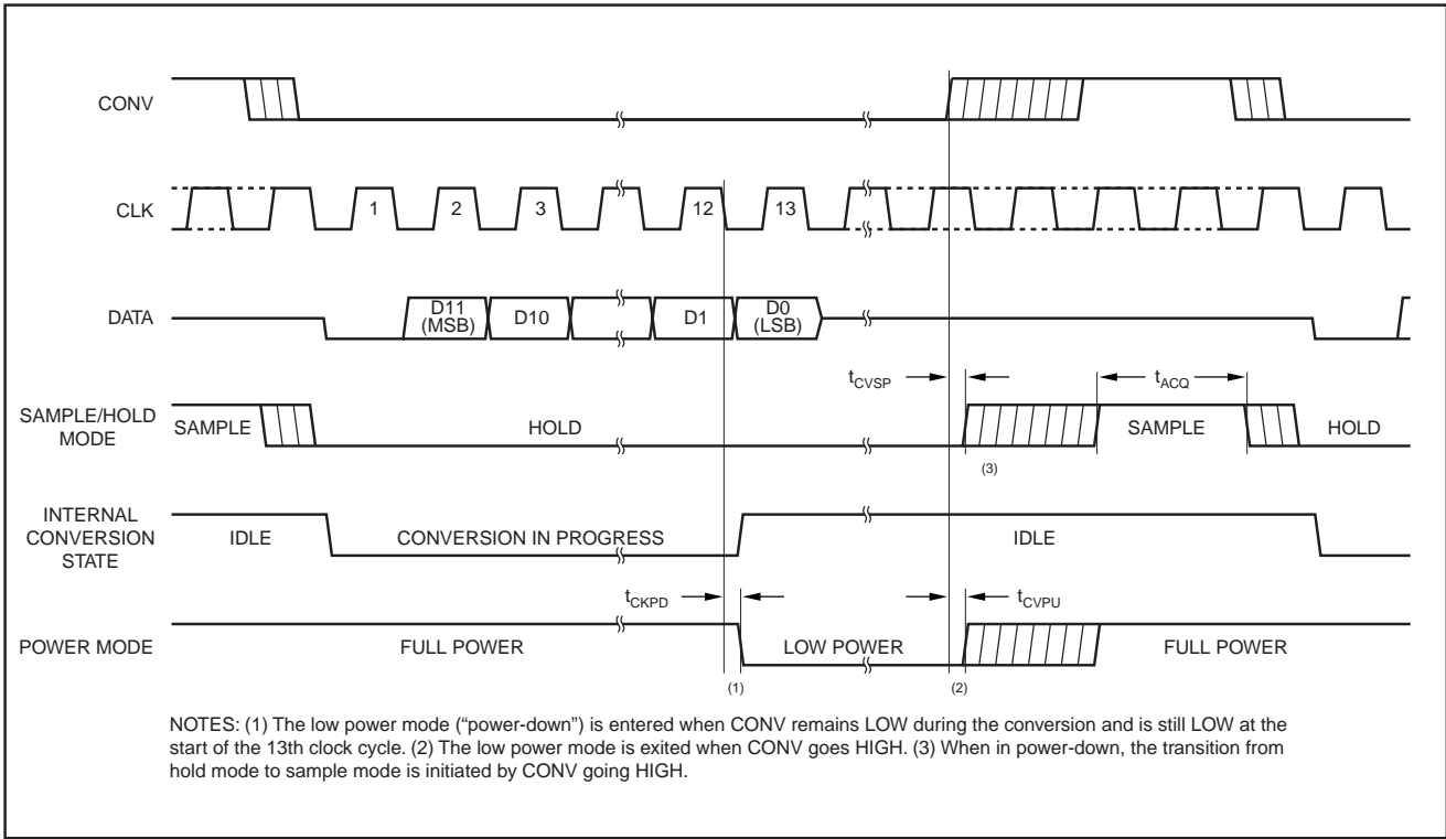
FIGURE 4. Power-Down Timing.
