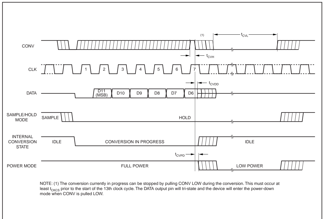
FIGURE 6. Short-Cycle Timing.
