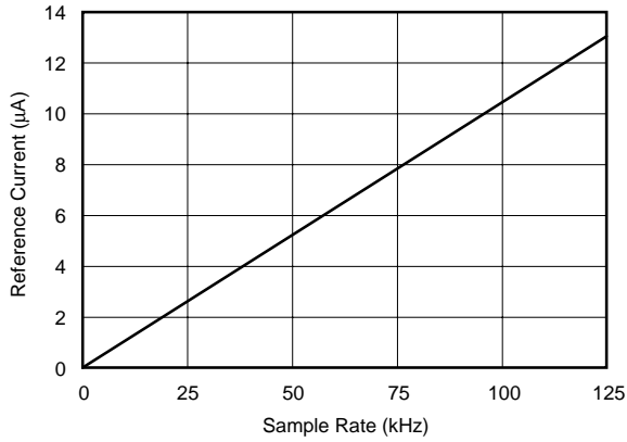
REFERENCE CURRENT vs SAMPLE RATE
