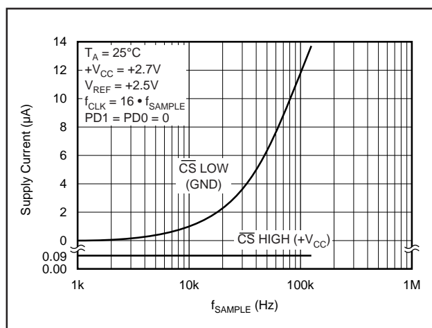
FIGURE 9. Supply Current vs State of \overline{CS} .
