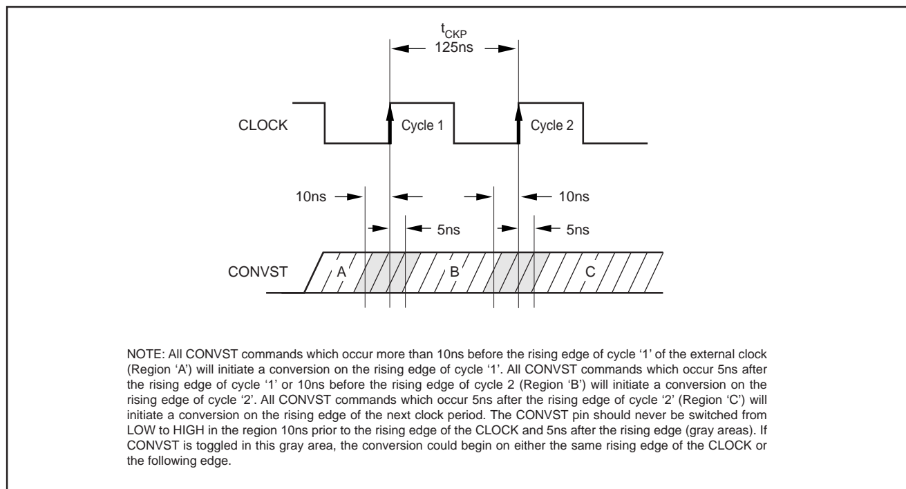
FIGURE 8. Conversion Mode.
