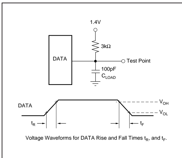
FIGURE 6. Test Circuits for Timing Specifications.
