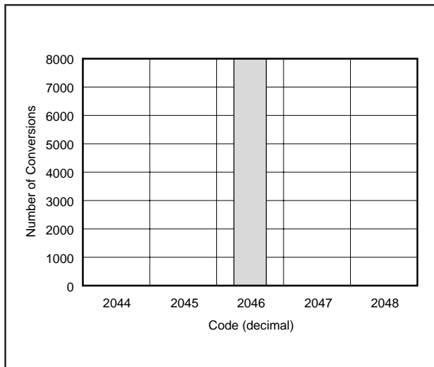
FIGURE 5. Histogram of 8,000 Conversions of a DC Input.
