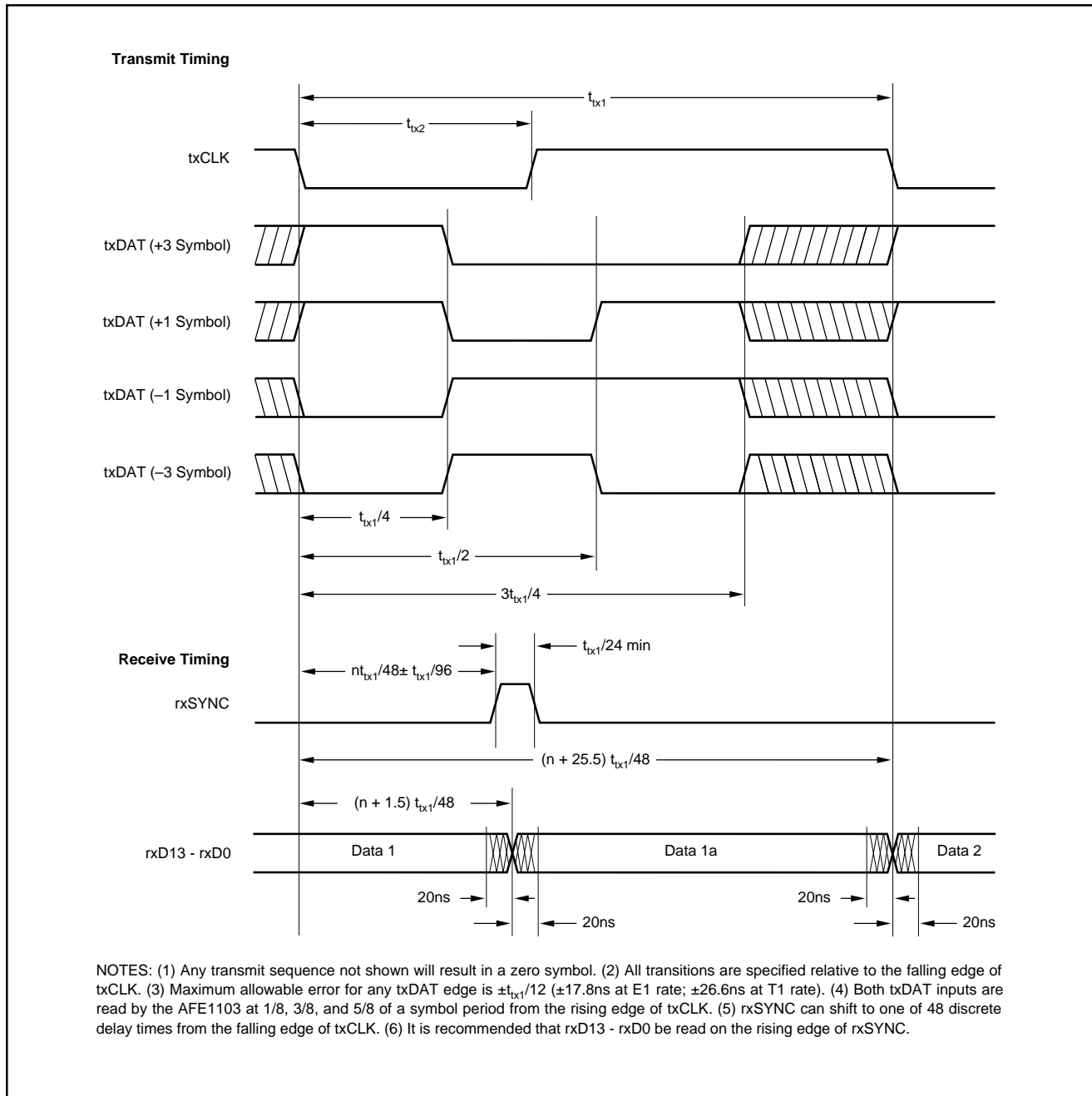
FIGURE 3. Timing Diagram.
