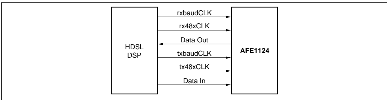
FIGURE 1. DSP Interface.
