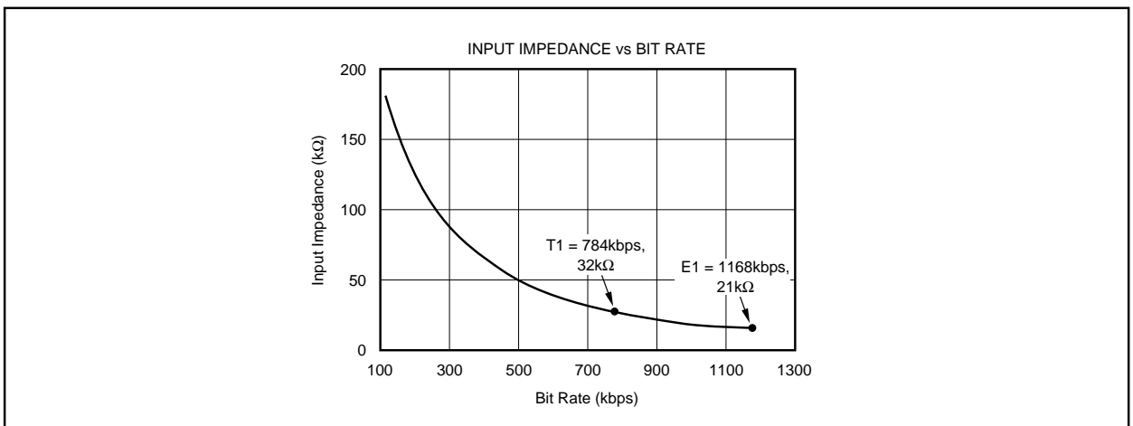
CURVE 3. Input Impedance of rxLINE and rxHYB.
