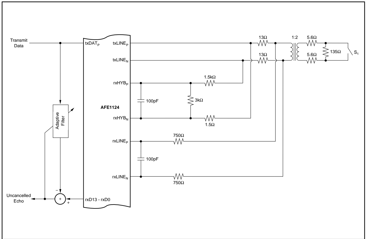
FIGURE 7. Uncancelled Echo Test Diagram.
