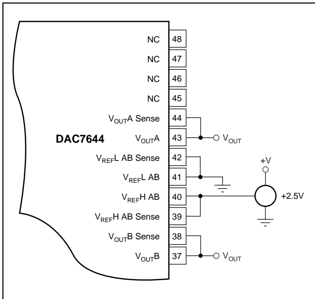
FIGURE 12. Low Cost Single-Supply Configuration.
