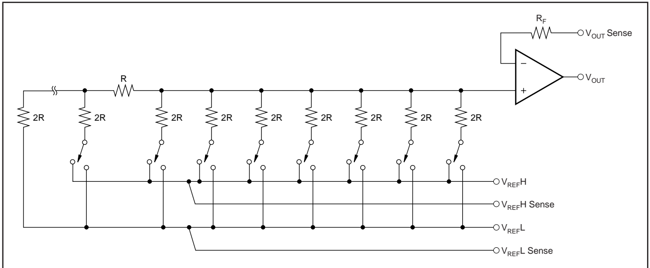
FIGURE 1. DAC7644 Architecture.
