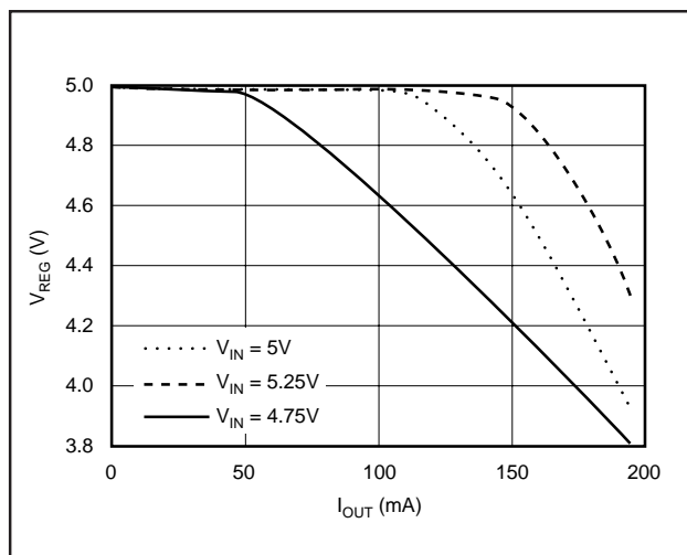
FIGURE 9. DCP010505P AND LP2986 Regulator.
