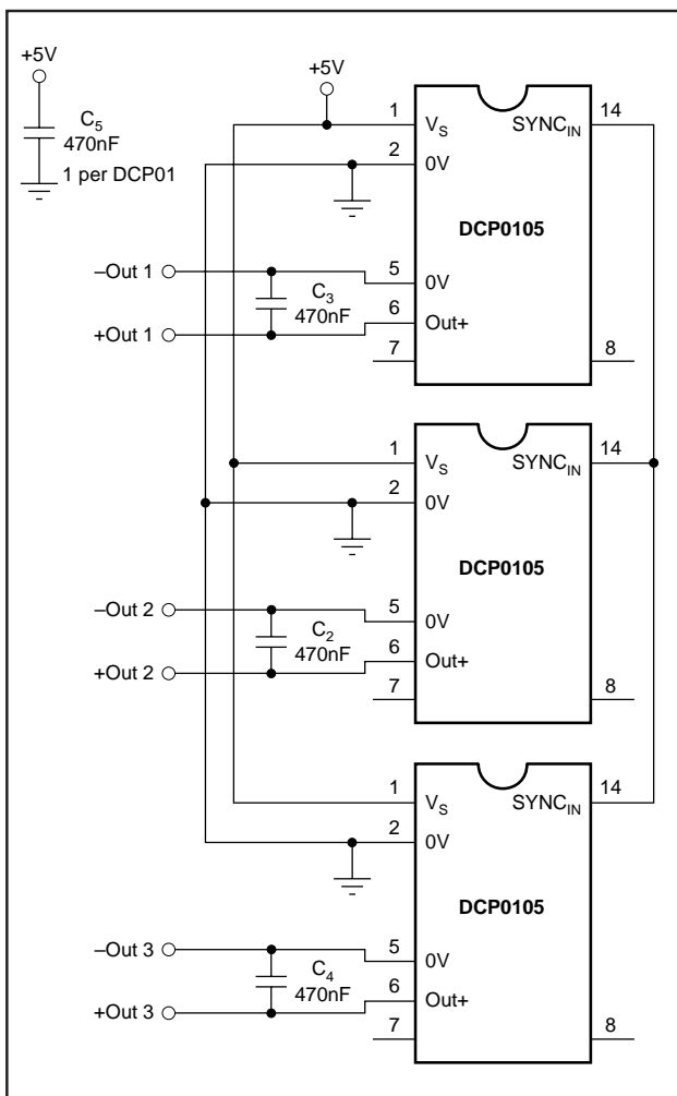
FIGURE 1. Standard Interface.
