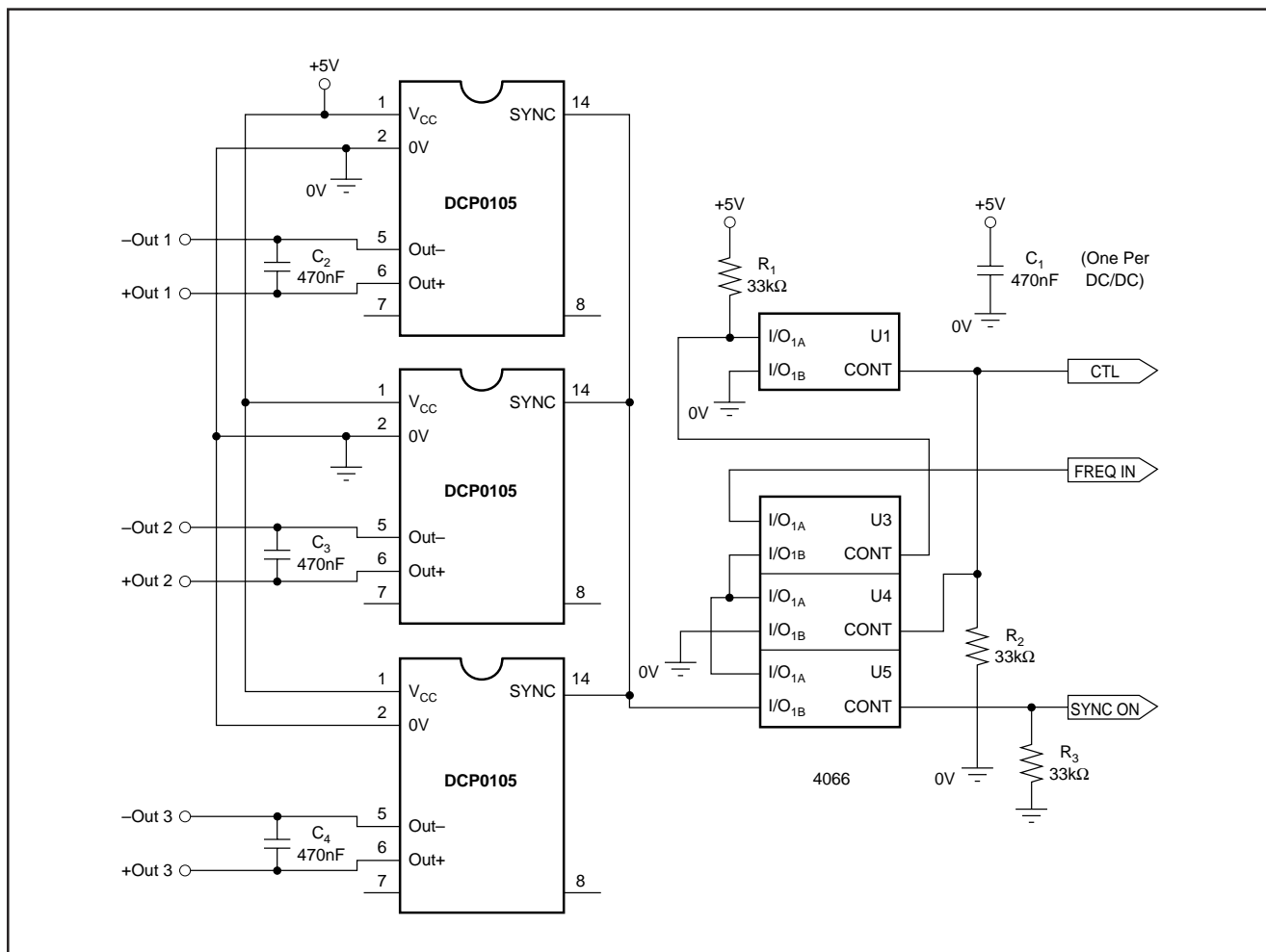
FIGURE 3. Universal Interface.
