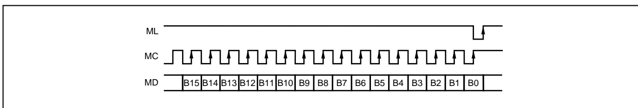
FIGURE 9. Software Interface Format.
