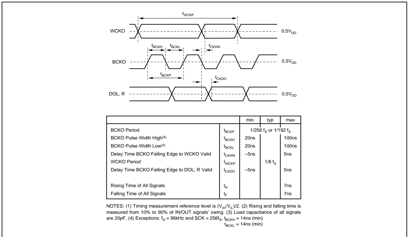
FIGURE 7. Audio Output Data Format.
