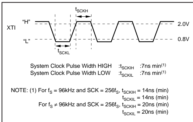
FIGURE 1. System Clock Timing.
