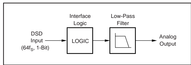
FIGURE 2. DSD Playback.
