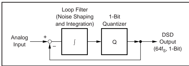
FIGURE 1. DSD Recording.
