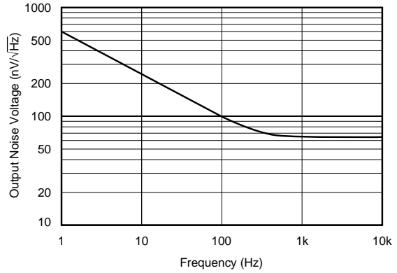
OUTPUT NOISE VOLTAGE vs FREQUENCY
