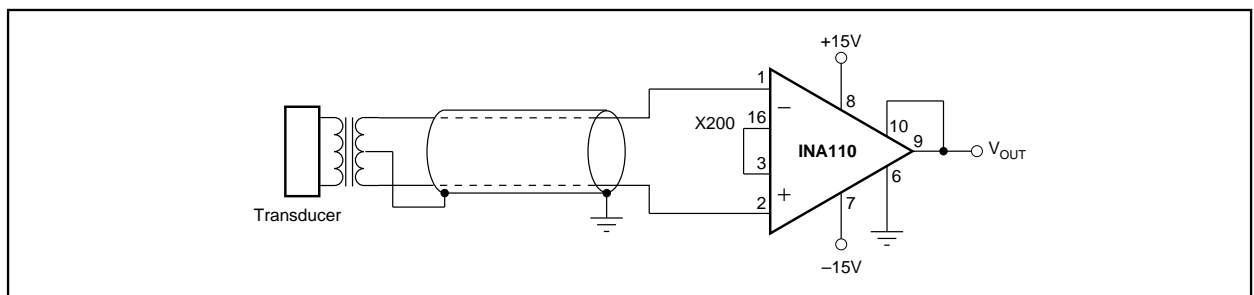
FIGURE 6. Transformer-Coupled Amplifier.
