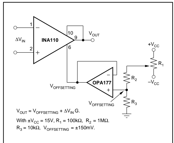
FIGURE 3. Output Offsetting.
