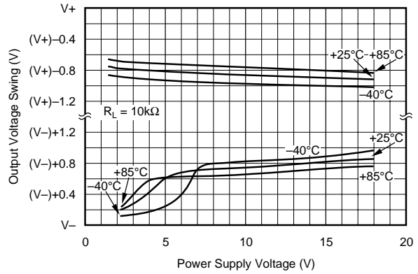
OUTPUT VOLTAGE SWING vs POWER SUPPLY VOLTAGE
