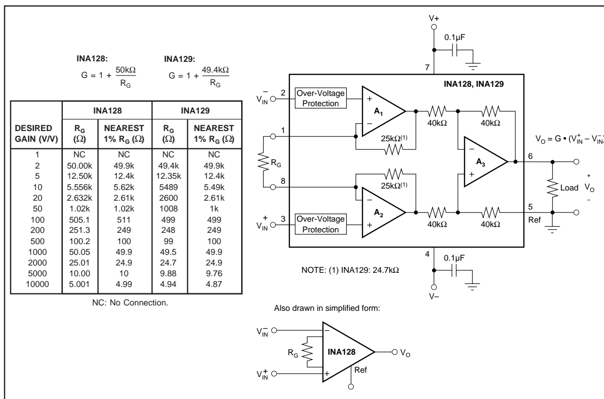
FIGURE 1. Basic Connections.
