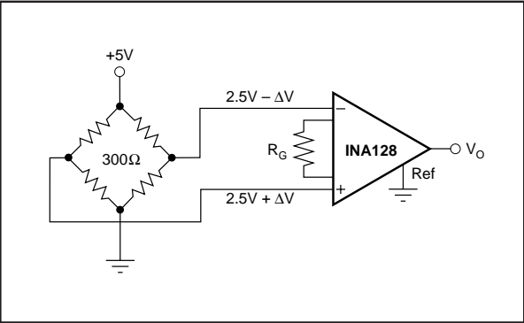
FIGURE 5. Bridge Amplifier.
