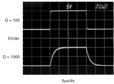
LARGE-SIGNAL STEP RESPONSE (G = 100, 1000)
