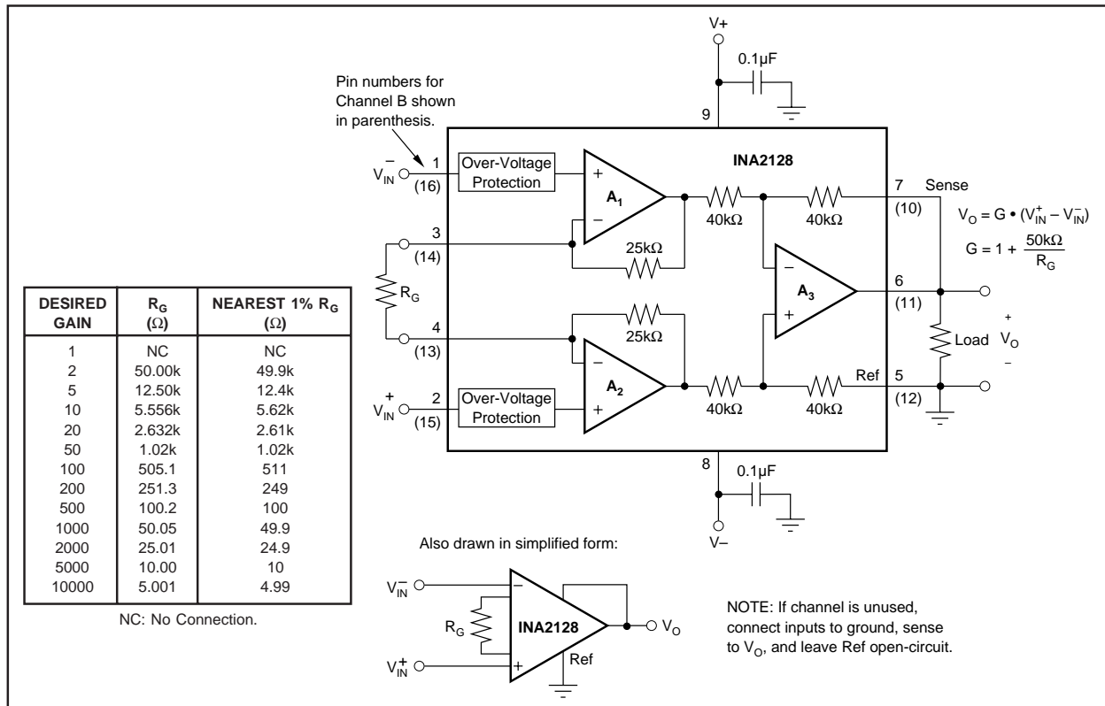
FIGURE 1. Basic Connections.
