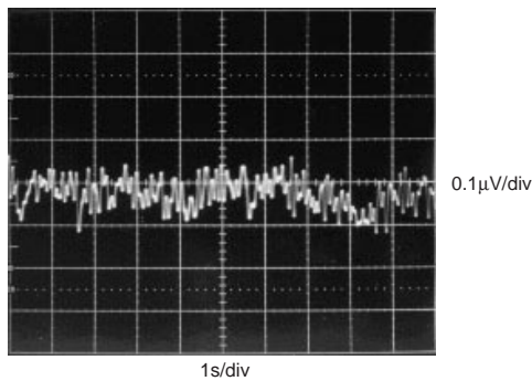
VOLTAGE NOISE 0.1 to 10Hz INPUT-REFERRED, G \geq 100
