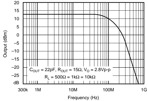
BANDWIDTH vs R_{LOAD}
