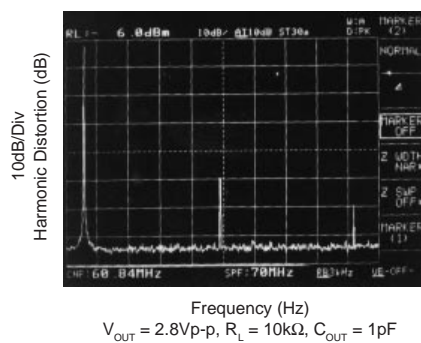
30MHz HARMONIC DISTORTION
