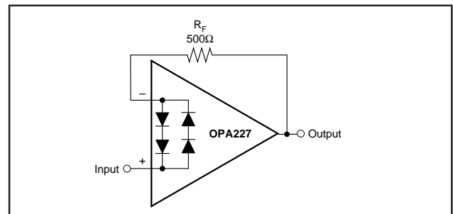
FIGURE 2. Pulsed Operation.
