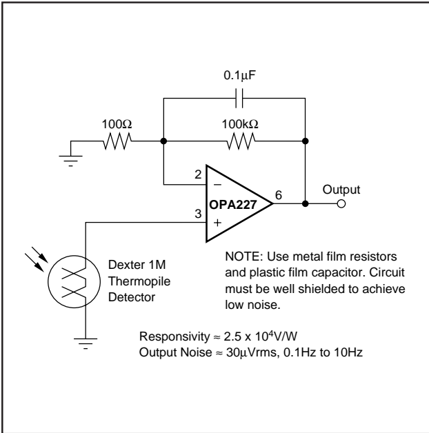
FIGURE 15. Long-Wavelength Infrared Detector Amplifier.
