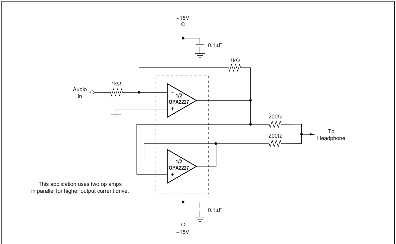
FIGURE 17. Headphone Amplifier.
