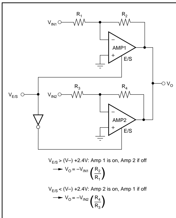
FIGURE 18. Switched Amplifier.
