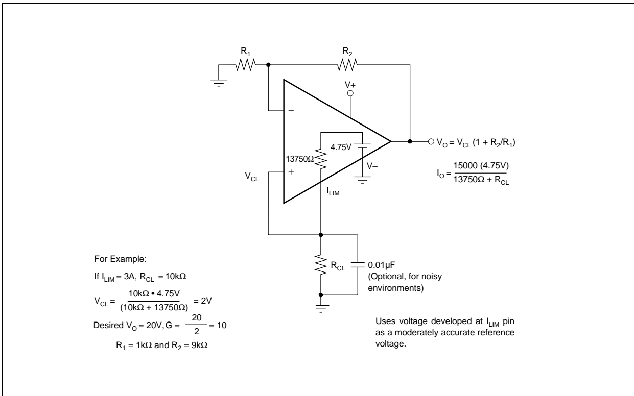
FIGURE 15. Voltage Source.
