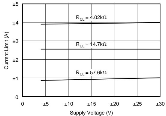
CURRENT LIMIT vs SUPPLY VOLTAGE
