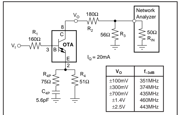
FIGURE 27. Forward Amplifier.
