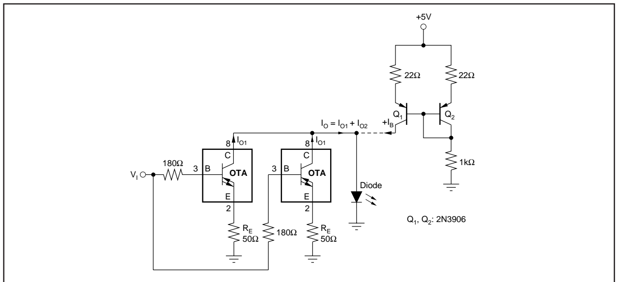
FIGURE 15. High Speed Current Driver.
