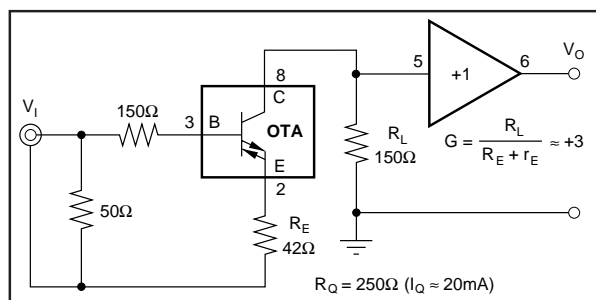
FIGURE 13. Cable Amplifier.
