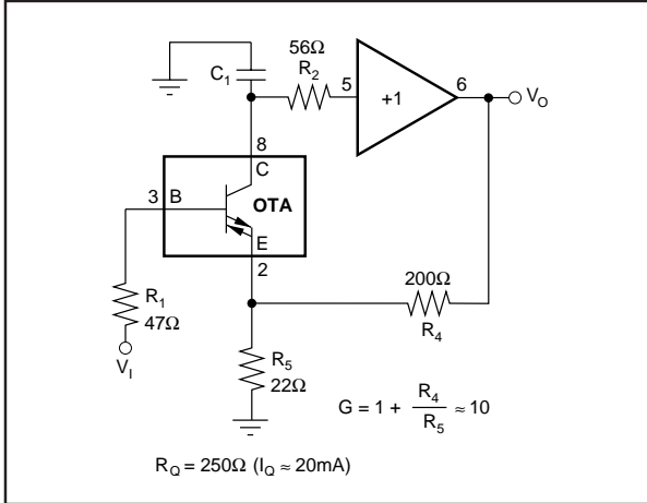
FIGURE 9. Current-Feedback Amplifier.
