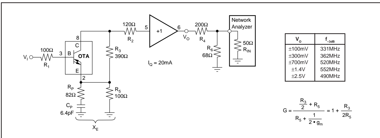
FIGURE 23. Direct-Feedback Amplifier.
