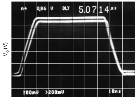
(HDTV Signal Pulse) t_R = t_F = 10\text{ns} , V_O = 5\text{Vp-p}
