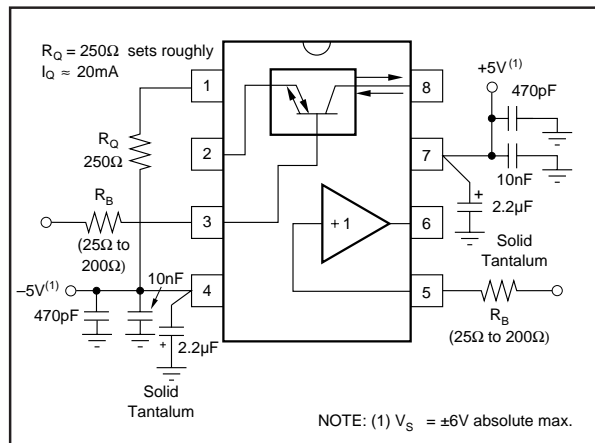
FIGURE 2. Basic Connections.
