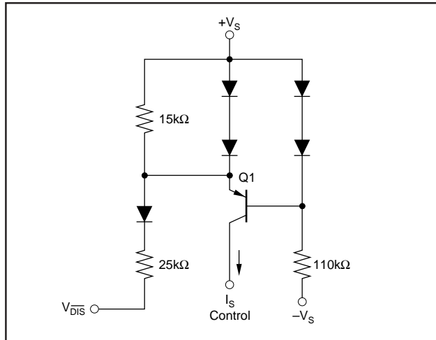
FIGURE 9. Simplified Disabled Control Circuit.
