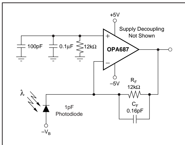
FIGURE 3. Wideband, High Sensitivity, OC-3 Transimpedance Amplifier.
