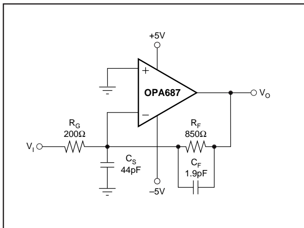
FIGURE 4. Broadband Low Inverting Gain External Compensation.
