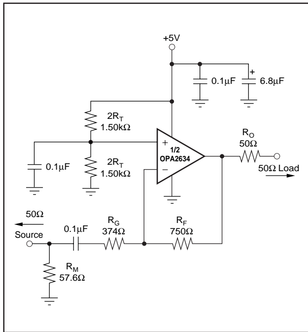
FIGURE 7. Gain of -2 Example Circuit.
