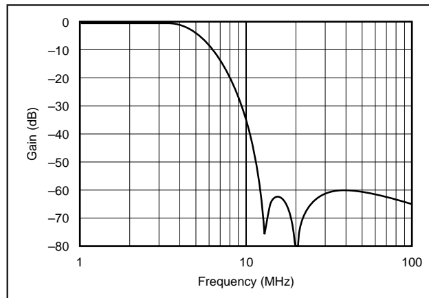
FIGURE 4. Nominal Filter Response.
